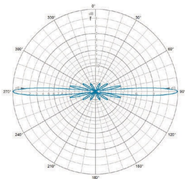
E-Plane | 875 MHz
