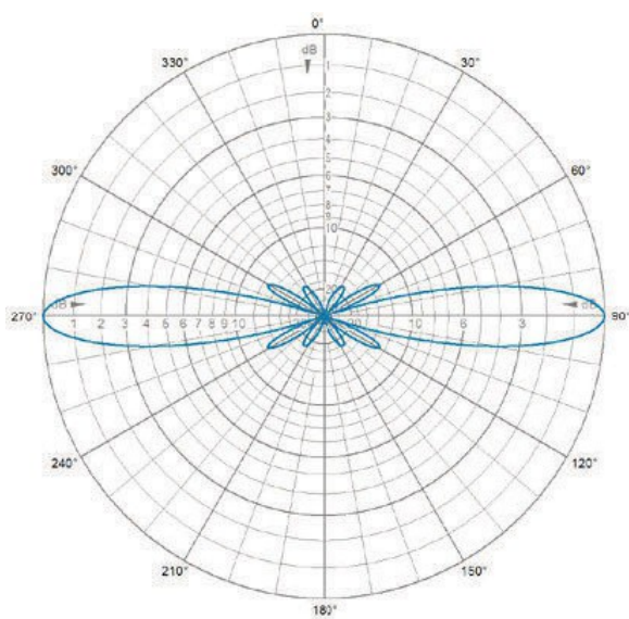
E-Plane | 435 MHz
