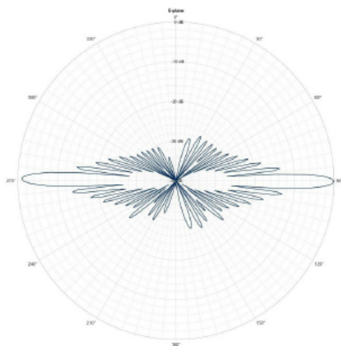
E-Plane, 915MHz
