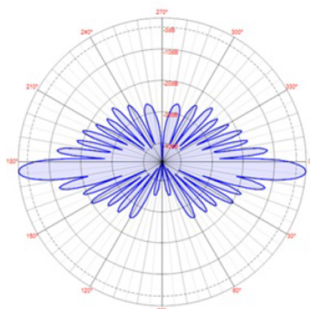
Elevation Pattern, 4°
