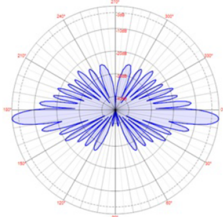
Elevation Pattern, 5°
