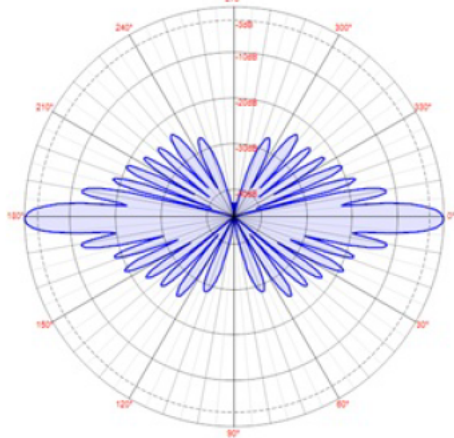
Elevation Pattern, 1°
